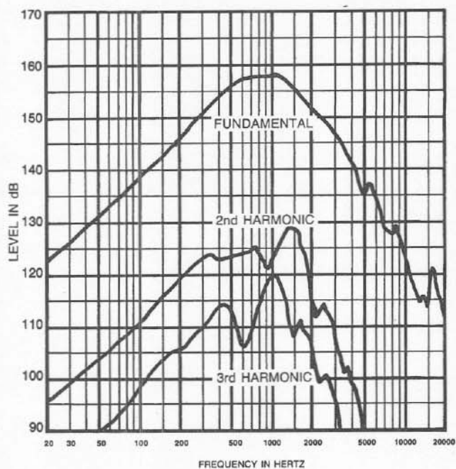
FIGURE 1 Distortion Response — Plane Wave Tube (1 inch) (7.5-watt input)
