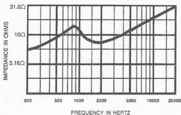
FIGURE 4 Impedance Response — Cobreflex III Horn
